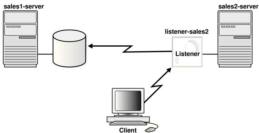
Figure 9-1 Remote Listener
